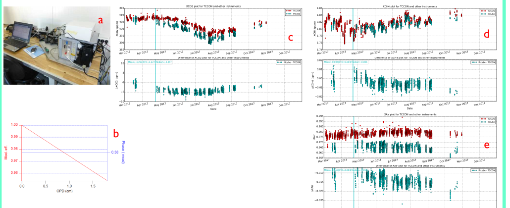
Fig. 6: (a) IRCube, (b) ILS parameters plot for IRCube, timeseries of XCO 2 , XCH 4 and XAir for the IRCube (cyan) and TCCON (red) (top panel of c-e) and the difference of IRCube relative to the TCCON (bottom panel of c-e).
