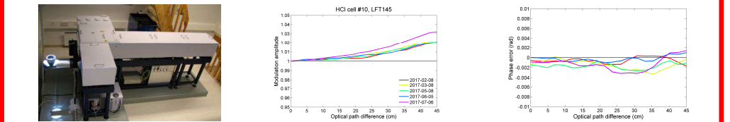
Fig. 3: (left) Bruker IFS 125HR at Sodankylä TCCON site, ILS parameters — modulation efficiency (center) and phase error (right) for the Bruker IFS 125HR.
