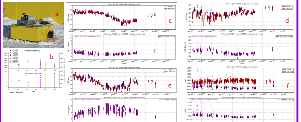
Fig. 5: (a) EM27/SUN, (b) ILS parameters plot for EM27/SUN, timeseries of XCO 2 , XCH 4 , XCO and XAir for the EM27/SUN (magenta) and TCCON (red) (top panel of c-e) and the difference of EM27/SUN relative to the TCCON (bottom panel of c-e).
