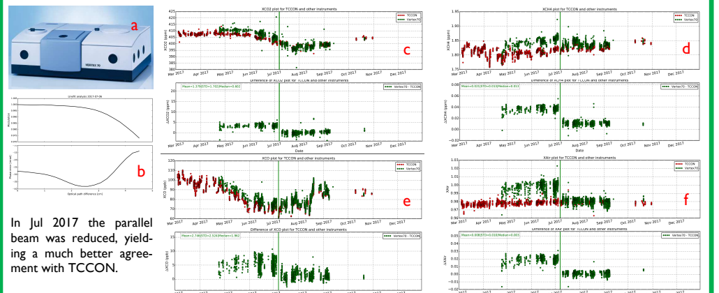
Fig. 4: (a) Vertex70, (b) ILS parameters plot for Vertex70, timeseries of XCO 2 , XCH 4 , XCO and XAir for the Vertex70 (green) and TCCON (red) (top panel of c-f) and the difference of Vertex70 relative to the TCCON (bottom panel of c-f).
